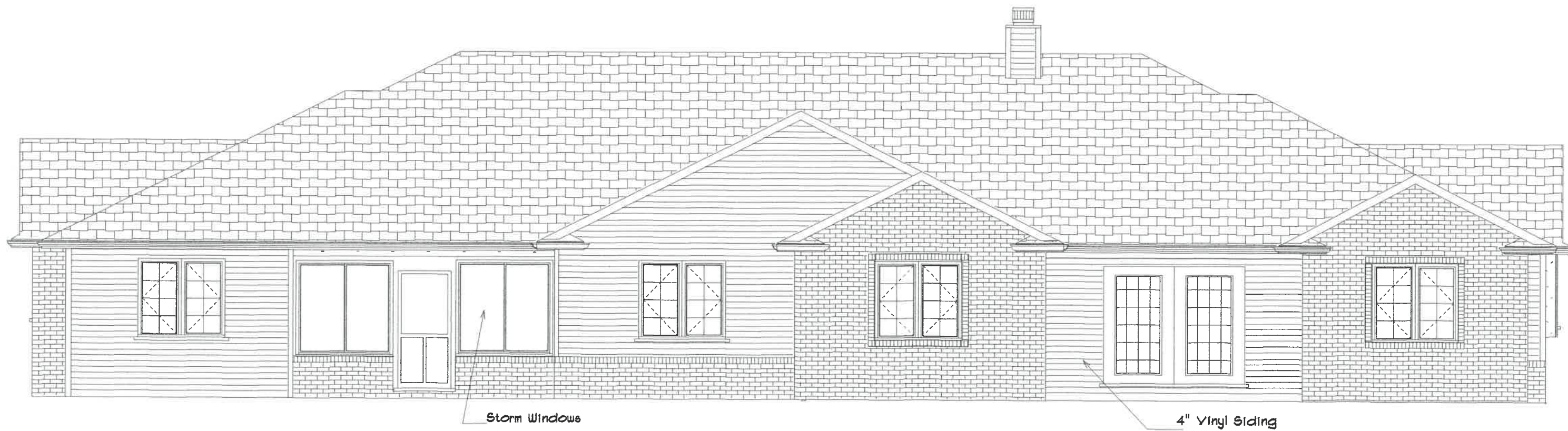
REAR ELEVATION
